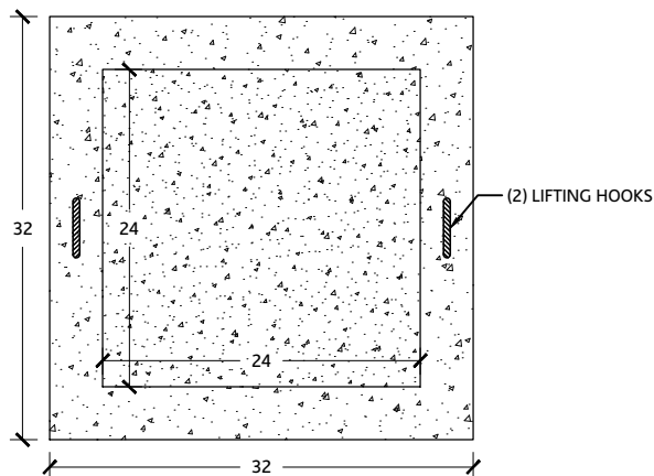
ELEVATION VIEW
