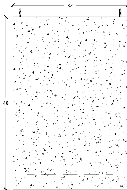
SECTION VIEW
